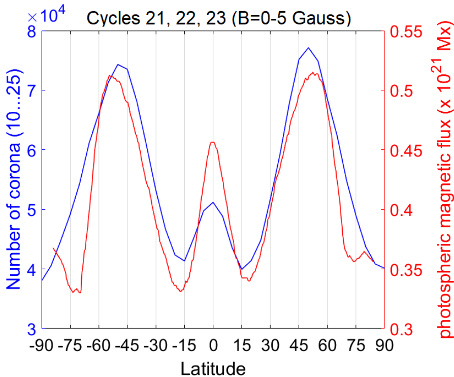
Figure 9. Number of HCDS corona events between 10–25 (blue) and photospheric magnetic flux (red) in Mx for magnetic fields between 0–5 Gauss.
