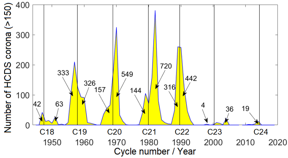
Figure 3. Number of HCDS indices greater than 150 for the Cycles 18–24. The black vertical lines show the maxima of the cycles.
