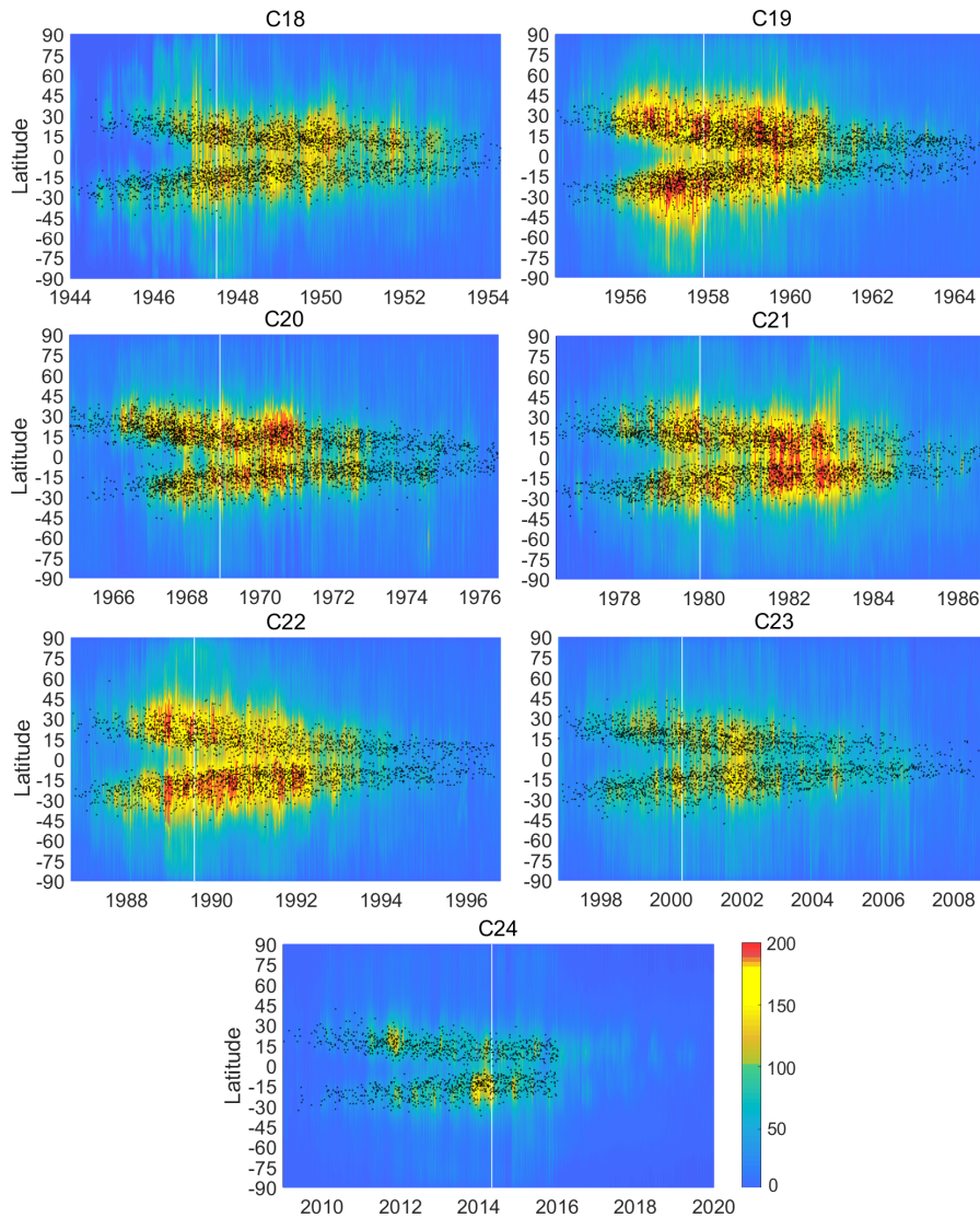
Figure 1. A combined figure of homogeneous corona data set (color bar) and sunspot groups (black dots) separately for Solar Cycles 18–24. The white vertical lines show the maxima of the cycles. (Note that sunspots for 2017-2019 are missing from the used database.)
