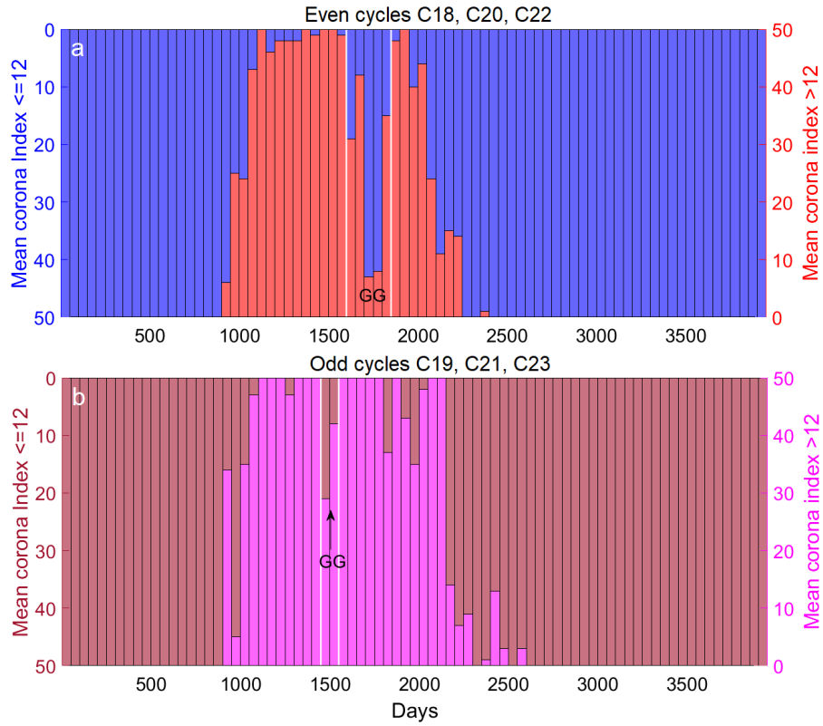
Figure 11. The amount of CI values \leq 12 or > 12 as a histogram for a) even and b) odd cycles between SC18–SC23.
