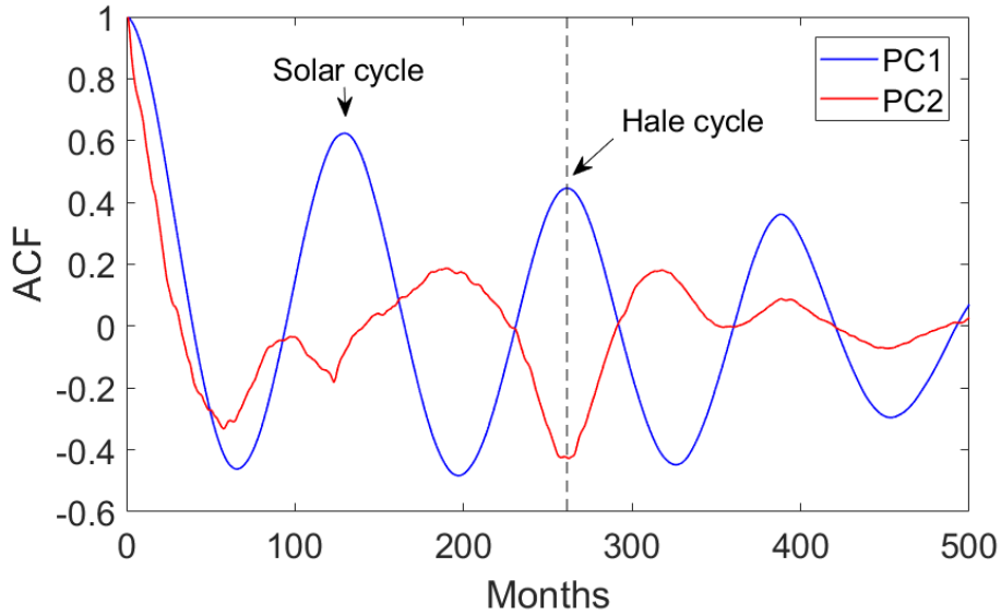
Figure 14. The autocorrelation functions of PC1 and PC2 timeseries of CI for Cycles 19–24. Note a deep minimum in the ACF of PC2 at Hale cycle period.
