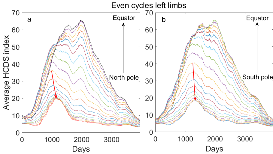
Figure 2. The lines (with 5-degree resolution) of the average HCDS indices in the left limb of the Sun as a function of day for the average even cycle. The lines are arranged such that the lowest lines are at poles and highest lines at equator. The red arrows show the temporal drift of the latitudinal maxima towards poles. Figs. 2a and b are for northern and southern hemisphere, respectively.
