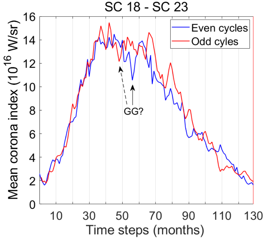
Figure 10. Average monthly CI for even and odd cycles of the period SC18–SC23
