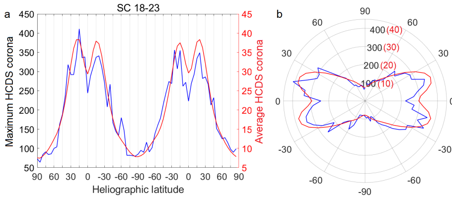
Figure 4. The maximum (blue, left vertical axis) and average values (red, right vertical axis) of HCDS for Solar Cycles 18–23 a) in Cartesian coordinates, and b) in polar coordinates. (Note that for polar coordinates maximum is black value and average red value.)
